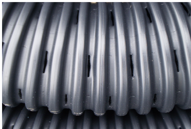
Perforated drain tile installed underground lets water seep into the subsoil.
